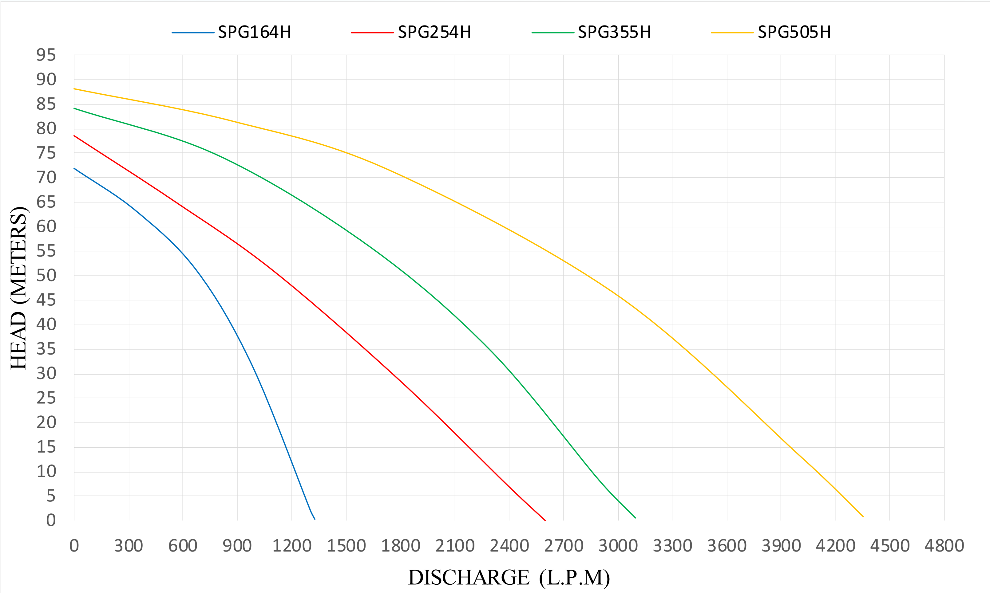
16 to 50 HP (High Head)
