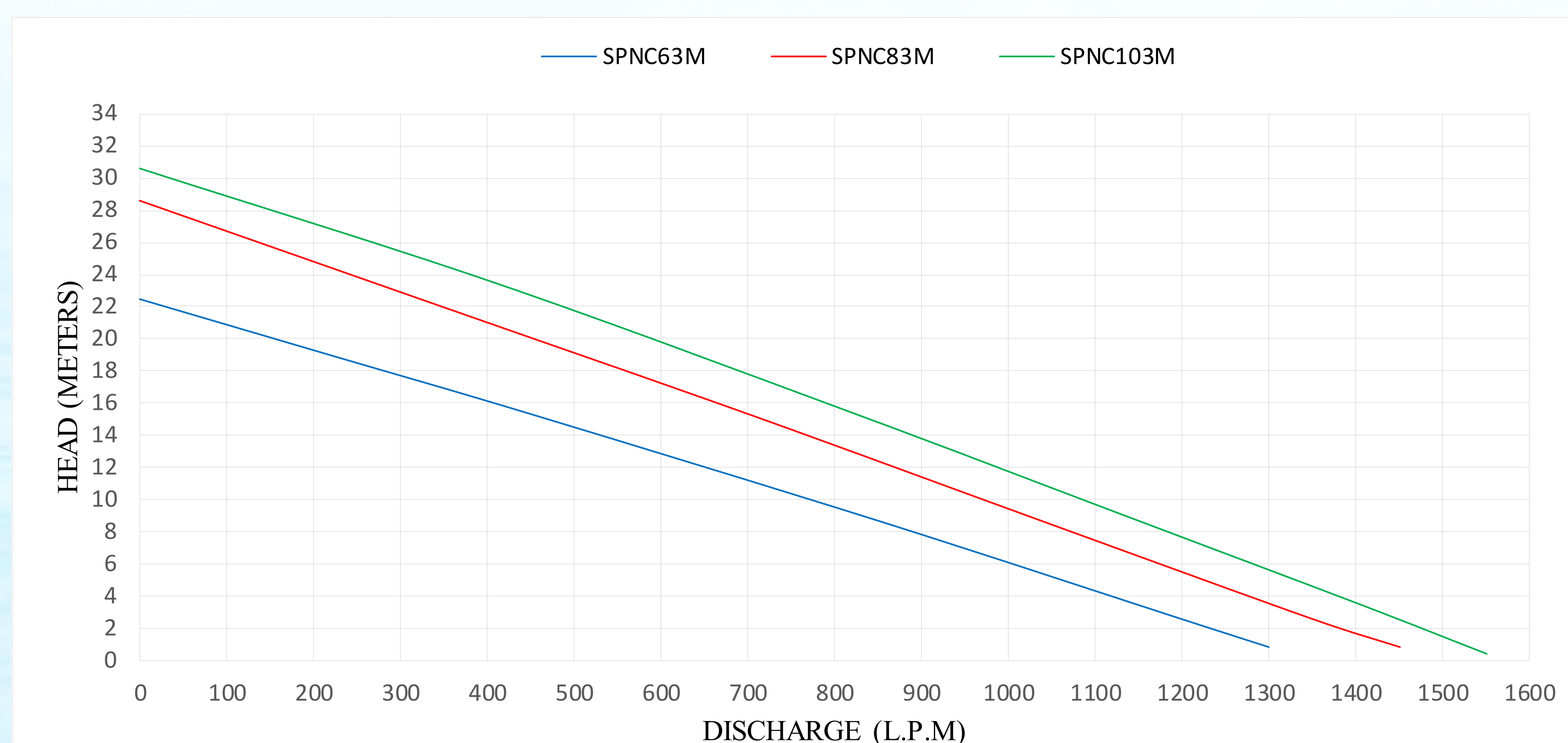
6 HP to 10 HP
