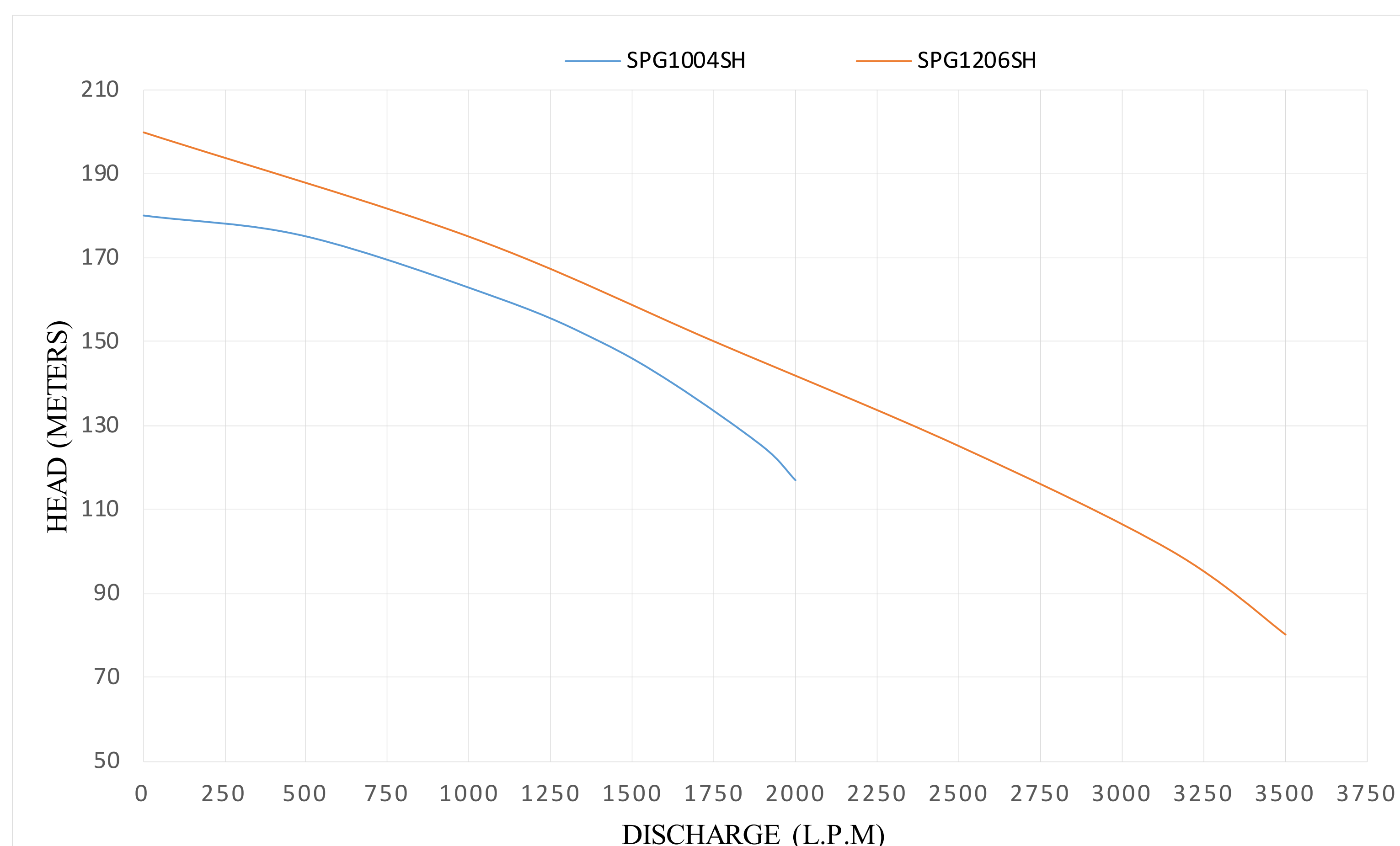
90 to 120 HP (Super Head)
