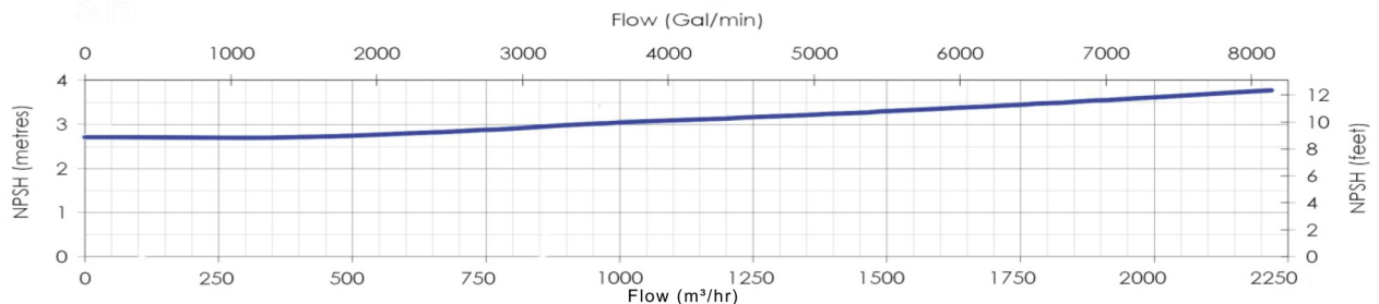
NPSH
