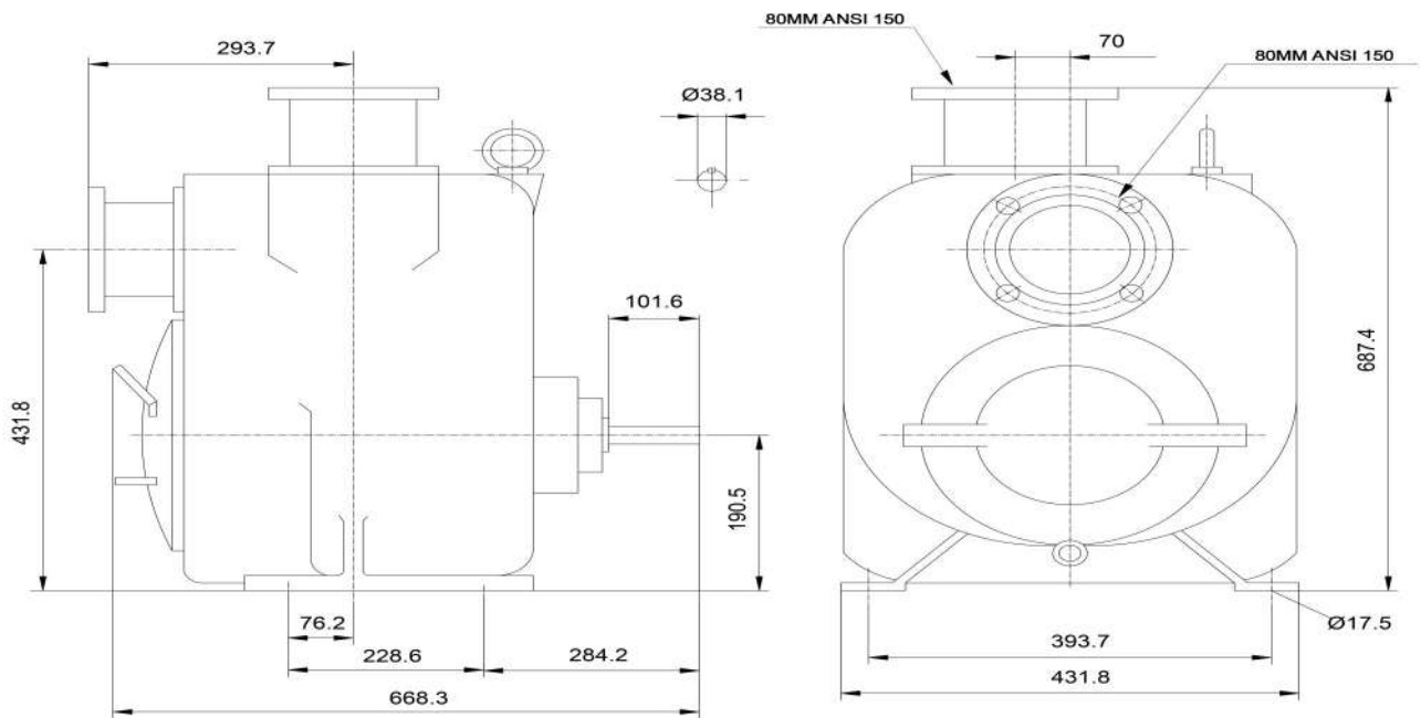
Approximate physical dimensions of pump model EDP-SP-3x3L
