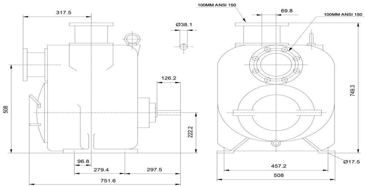
Approximate physical dimensions of pump model EDP-SP-4x4H
