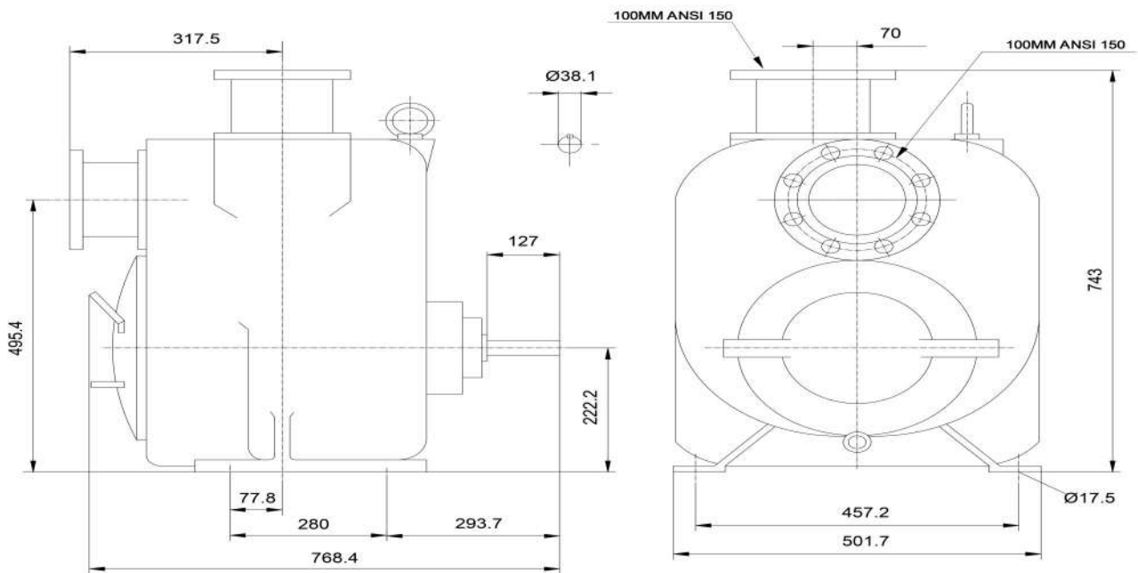
Approximate physical dimensions of pump model EDP-SP-4x4L
